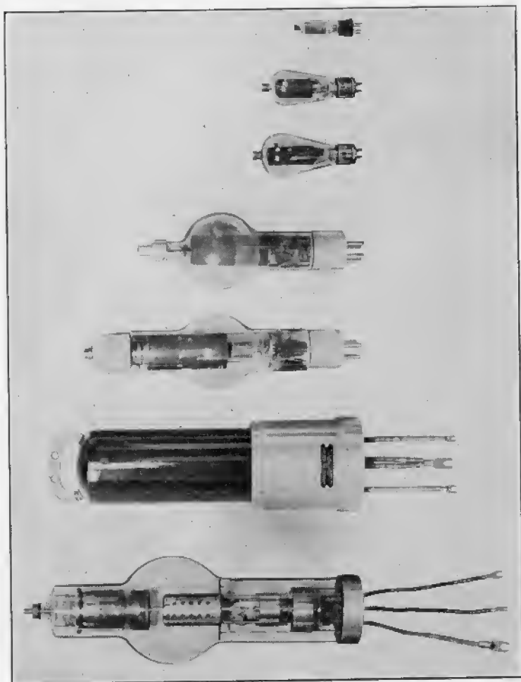
Fig. 6. A group of three-electrode, mercury-vapor-filled tubes. The ratings of these tubes range from 15,000 volts and 75 amperes down to 1,000 volts and 0.125 amperes.
